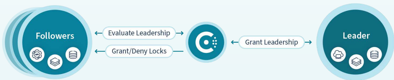
Coordinating leadership changes between nodes
