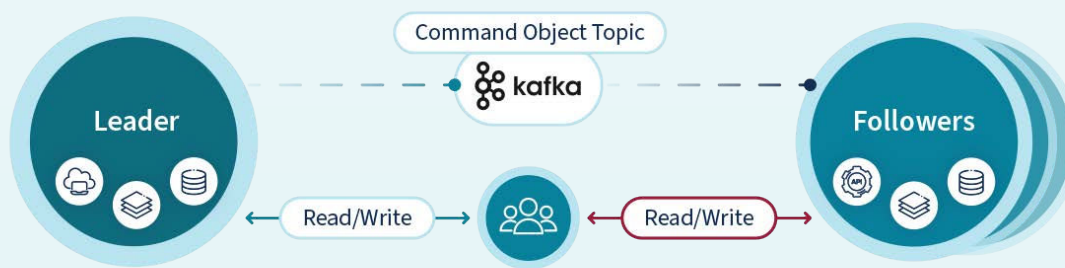
Distributed architecture – Refactoring write operations
